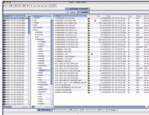
MacOS
